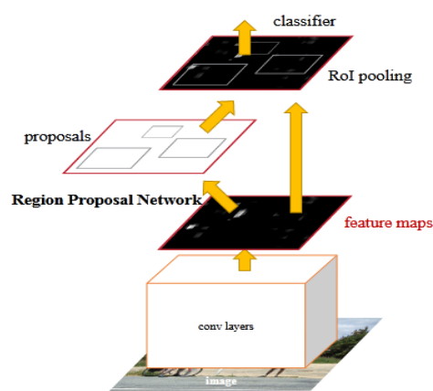
Figure. Faster RCNN.
